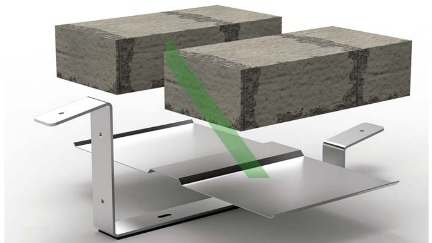
Fig.2: Ballast Tray installation option
