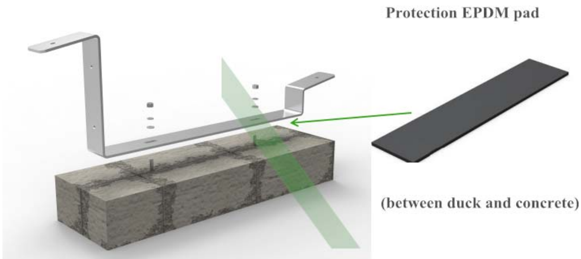
Fig.3: Concrete Block Installation option
